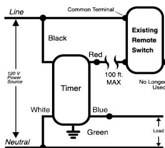
TYPICAL THREE-WAY WIRING
