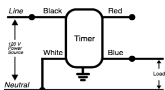
SINGLE-POLE WIRING
