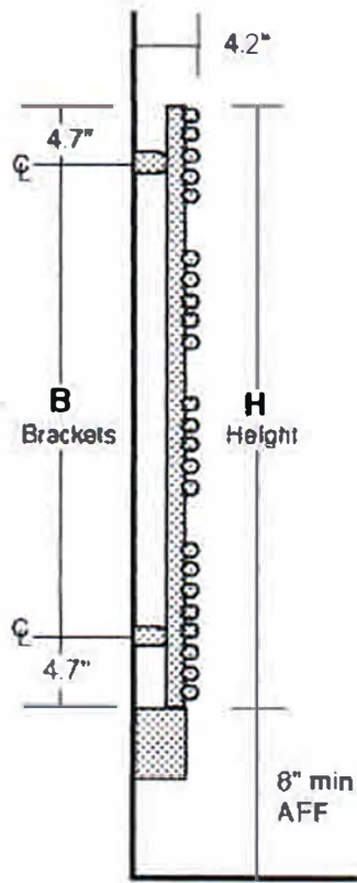
Side View Dimensions
