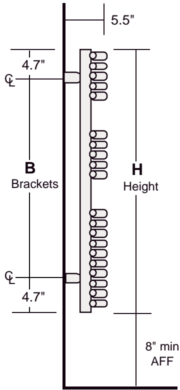
Side View Dimensions
