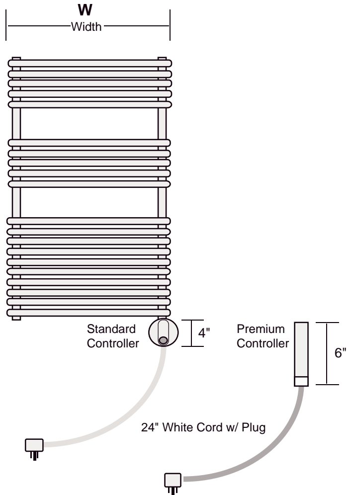
Front View Dimensions
