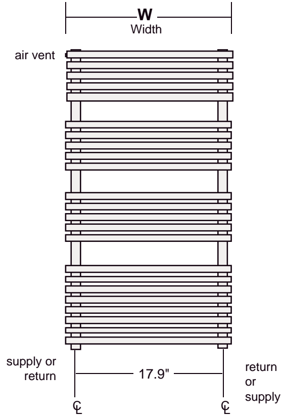
Front View Dimensions
