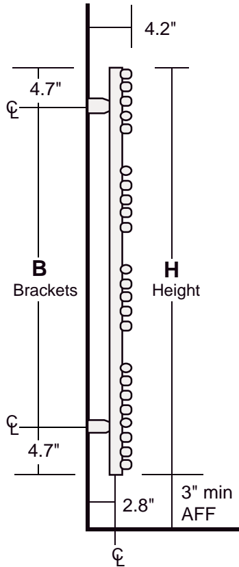
Side View Dimensions
