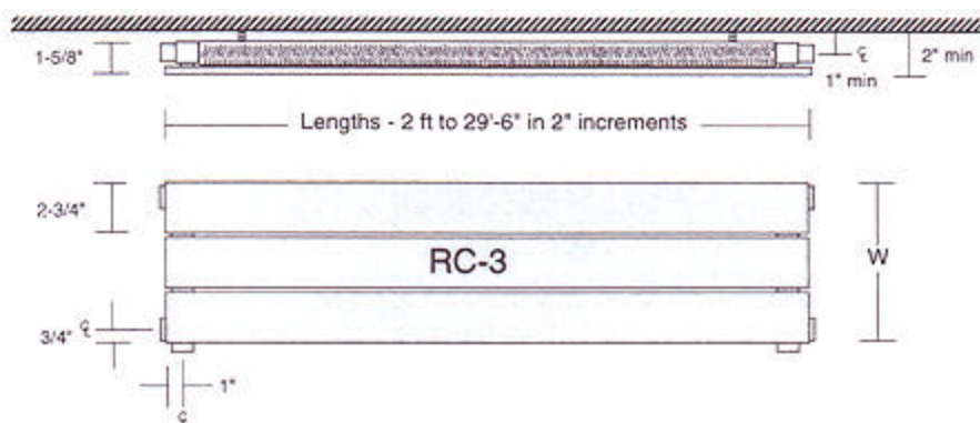
RC-3 with Both Side & Vertical Connections - Shown for Example Only
