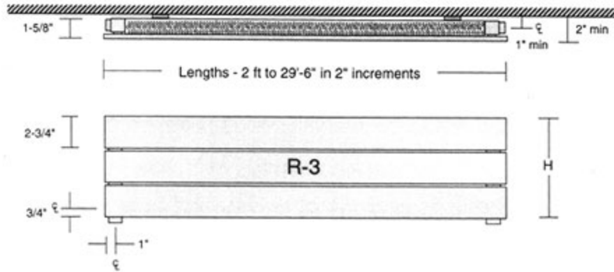
R-3 with Both Side & Vertical Connections - Shown for Example Only
