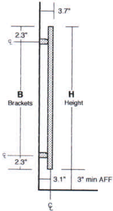
Side View Dimensions
