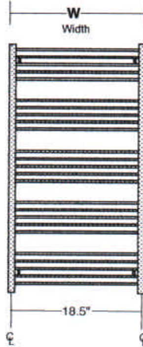
Front View Dimensions
