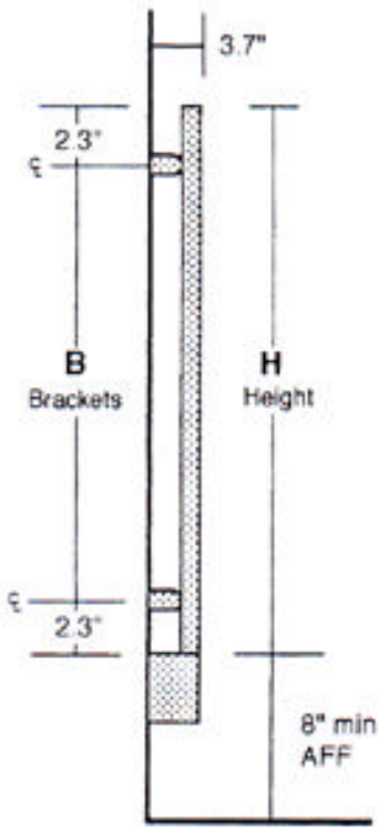
Side View Dimensions
