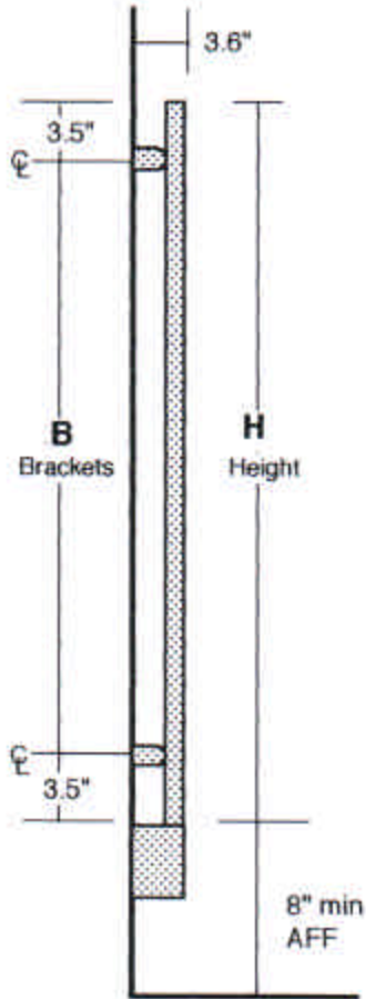
Side View Dimensions
