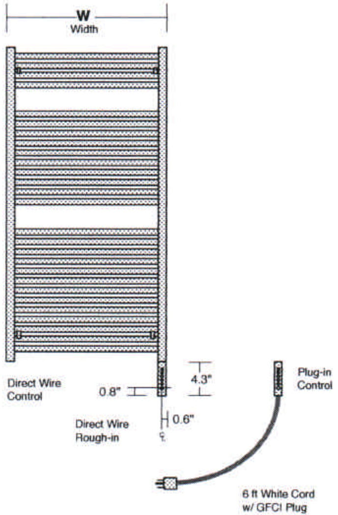
Front View Dimensions
